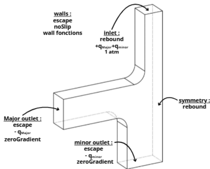
Figure 3.3: Named selection with their respective boundary conditions.
