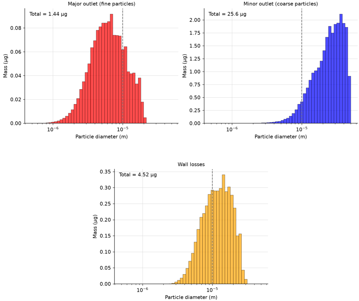
Figure 4.6: Mass distribution diagram of the optimized set of parameters for each outlet. The dotted line represents the aimed d_{50} .
