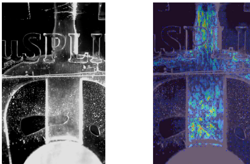
Figure B.1: Comparison between the video and the PIV analysis, the measurement is about particles speed here, with the software PIVLAB
