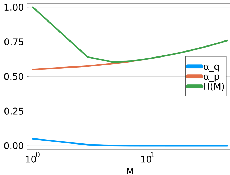
Figure S 1. Quantities \alpha_p , \alpha_q and \langle H \rangle as a function of the number of leaves M (odd values only). \alpha_p is increasing from 1/2 + \varepsilon to 1 while \alpha_q is decreasing from \varepsilon to 0. The average Hamming distance (L - 1)\alpha_q(M) + \alpha_p(M) reaches a minimum for an intermediate number of leaves. Values of parameters: \varepsilon = 0.05 , L = 10 .
