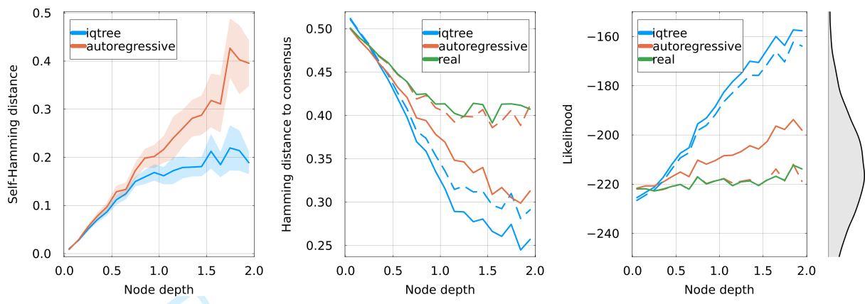
FIG. 2. Left: for Bayesian reconstruction, average pairwise Hamming distance among sequences reconstructed for each internal node. This quantifies the diversity of sequences obtained using Bayesian reconstruction. Center: Hamming distance between reconstructed sequences and the consensus sequence of the alignment. Solid lines represent maximum likelihood reconstruction or the real internal sequences, and dashed lines Bayesian reconstruction. IQ-TREE appears more biased towards the consensus sequence. Right: Log-likelihood of reconstructed and real sequences in the autoregressive model, i.e. using the logarithm of Eq. 2. Maximum likelihood methods (orange and blue solid lines) are biased towards more probable sequences. Bayesian autoregressive reconstruction gives sequences that are at the same likelihood level than the real ancestors. The equilibrium distribution of likelihood of sequences generated by Eq. 2 is shown on the right.
