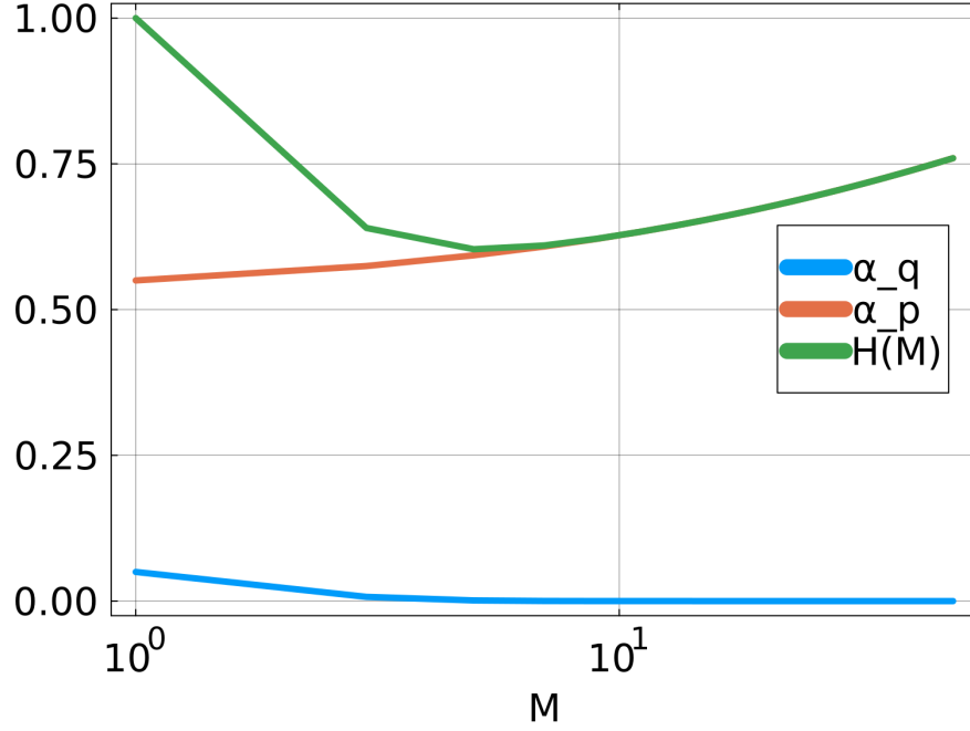
Figure S 1. Quantities \alpha_p , \alpha_q and \langle H \rangle as a function of the number of leaves M (odd values only). \alpha_p is increasing from 1/2 + \varepsilon to 1 while \alpha_q is decreasing from \varepsilon to 0. The average Hamming distance (L - 1)\alpha_q(M) + \alpha_p(M) reaches a minimum for an intermediate number of leaves. Values of parameters: \varepsilon = 0.05 , L = 10 .
