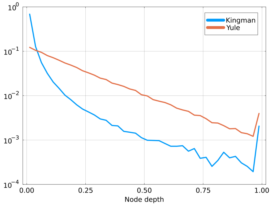
Figure S 3. Distribution of node depth for trees coming from the Kingman and Yule coalescents. Node depth is defined as the distance from a node to the closest leaf. Data is obtained by sampling several trees from each coalescent. Heights of trees are normalized to one. The Kingman process concentrates most of the nodes in close vicinity to the leaves, while the Yule process spreads them more evenly.
