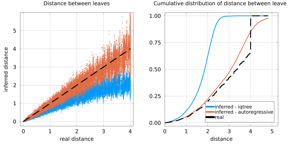
Figure S 2. Quality of branch length inference using data simulated with the autoregressive evolver and a tree with fixed topology. Two techniques are compared: IQ-TREE and the profile model corresponding to the autoregressive evolver. Left: inferred distance vs distance in the real trees for every pair of leaves. Right: Cumulative distribution of pairwise distance along the tree between leaves for the two inference methods and for the real tree. The discontinuity in the curve for the real tree is caused by the ultrametricity and fixed total height of the generated trees.
