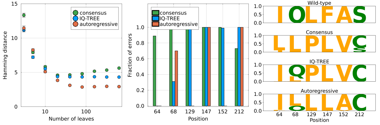
FIG. 4. Reconstruction of the wild-type PSE1 sequence used in [37] using sequences from round 20 of the directed evolution. Left. Non normalized Hamming distance to the wild-type PSE1 sequence as a function of the number of sequences M used for reconstruction. The fact that the consensus method has a local minimum is discussed in the Supplementary Material . For comparison, the average distance between a leaf sequence and the wild-type is 25. The error bars are computed using the standard deviation obtained from the 100 choices of sequences. Middle. For the six sequence positions where most of the reconstruction errors are located, fraction of errors of each method out of 100 independent reconstructions using different sets of M = 640 leaves. Right. Sequence logo of the reconstructed sequence for the three methods, obtained using 100 independent reconstructions with different sets of M = 640 leaves. The logo is only shown for the six positions where most errors are located. For example, all three methods fail 100 times at position 147, reconstructing a leucine L instead of a phenylalanine F .
