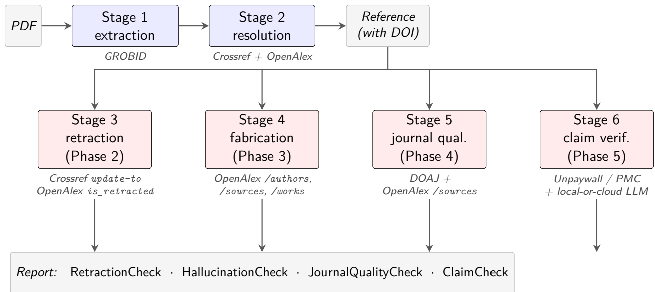
Figure 1: Citecheck’s six-stage pipeline. Stages 1–2 (blue) extract a typed Reference from the input PDF. Stages 3–6 (red) run in parallel against that Reference , each producing a typed check result. The aggregated report is the union of those four check results, one per citation-integrity failure mode. APIs consulted by each stage are labeled in italics; each stage is a separately replaceable module in src/citecheck/ .
