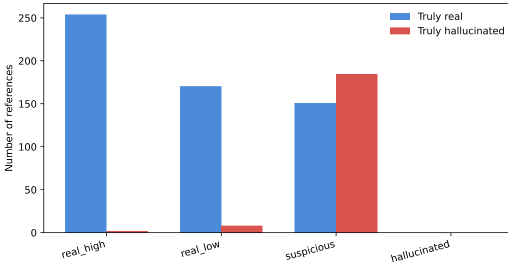
Figure 1: Predicted verdicts stratified by ground-truth class. The detector concentrates real references in real_high_confidence and real_low_confidence ; fabricated references either escalate to suspicious / likely_hallucinated (true positives) or fall into real_low_confidence (false negatives, almost all books).
