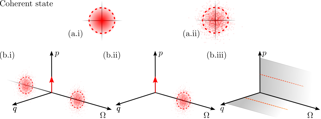
Coherent state
