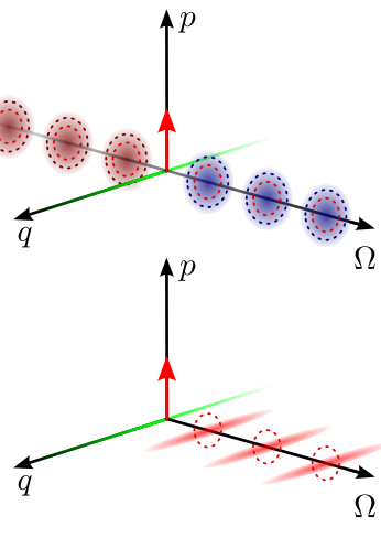
(c) Amplitude Squeezing
