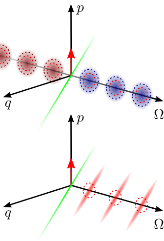
(b) Arbitrary Squeezing
