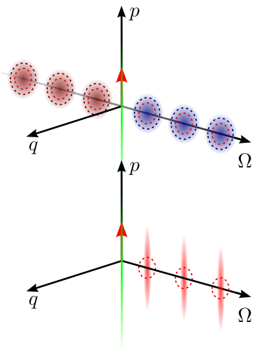
(a) Phase Squeezing
