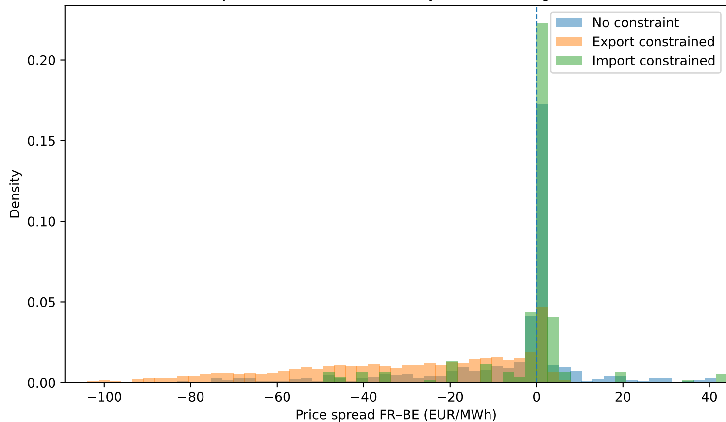
Spread distribution FR-BE by constraint regime
