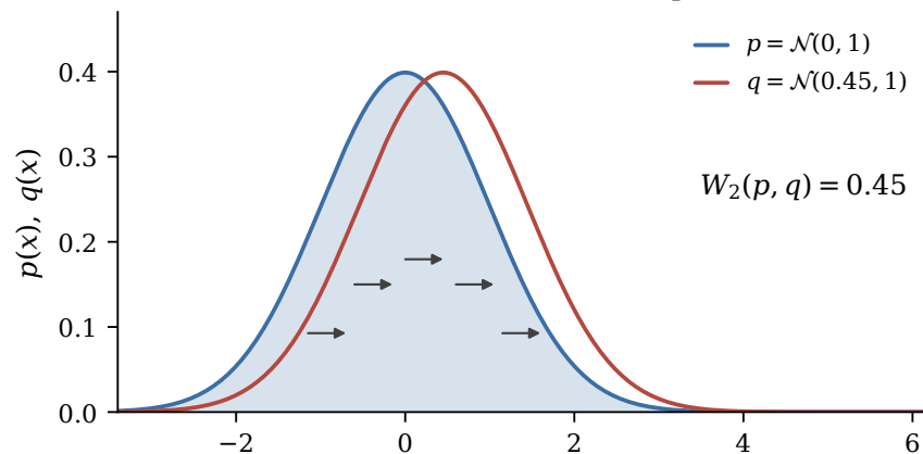
Wasserstein: short transport
