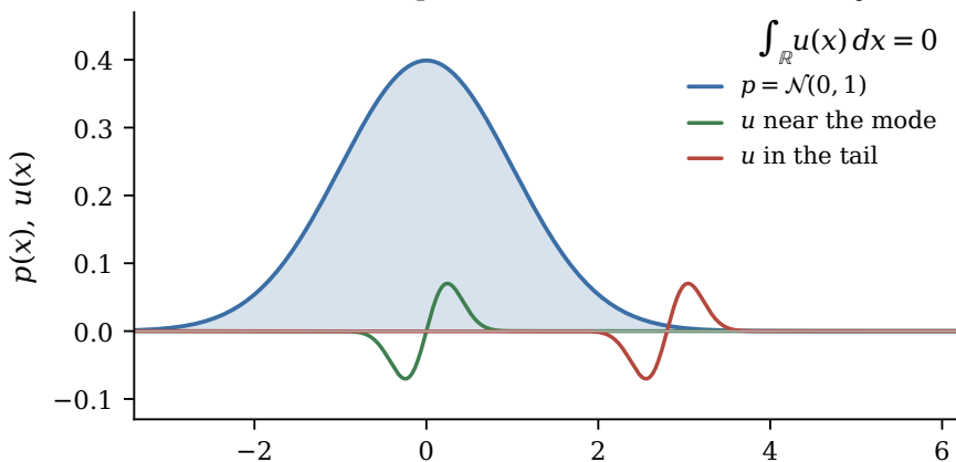
Fisher-Rao: same perturbation, different density level
