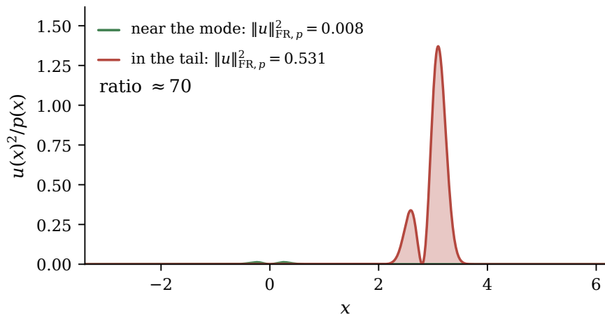
Fisher-Rao local energy density u^2/p
