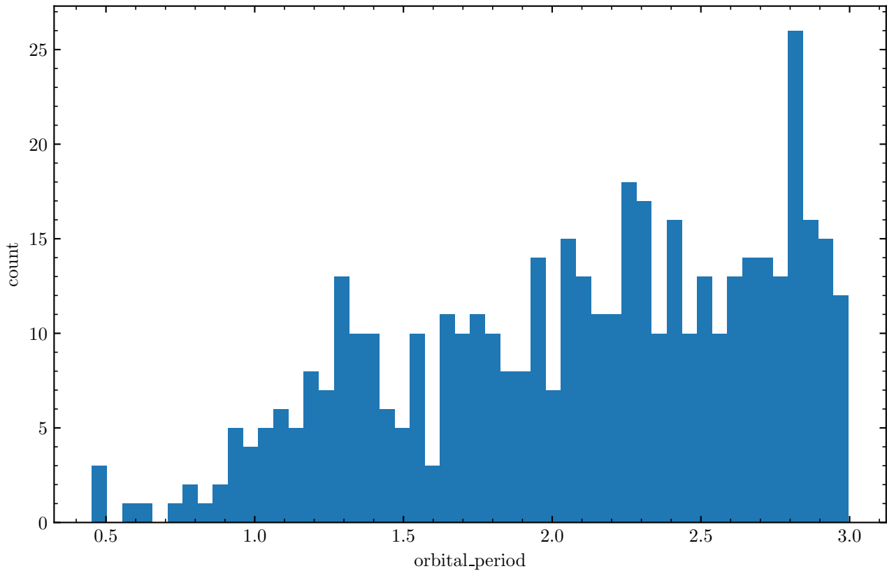
orbital_period of BH-Sol systems at inital detached state
