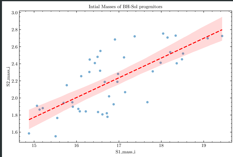
Figure 7: Initial ZAMS masses of simulation two, with mass ratios from Moe17PsandQs. Note that two failed systems have been excluded
