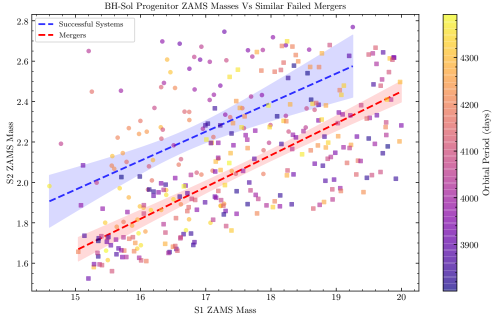
Figure 1: Here we can see that there seems to be a (quite rough) survival line based on the initial mass ratio and the orbital period. Note that these were simply constrained based on the max and min of the initial masses. Next step is actually sampling from a proper matching distribution.
