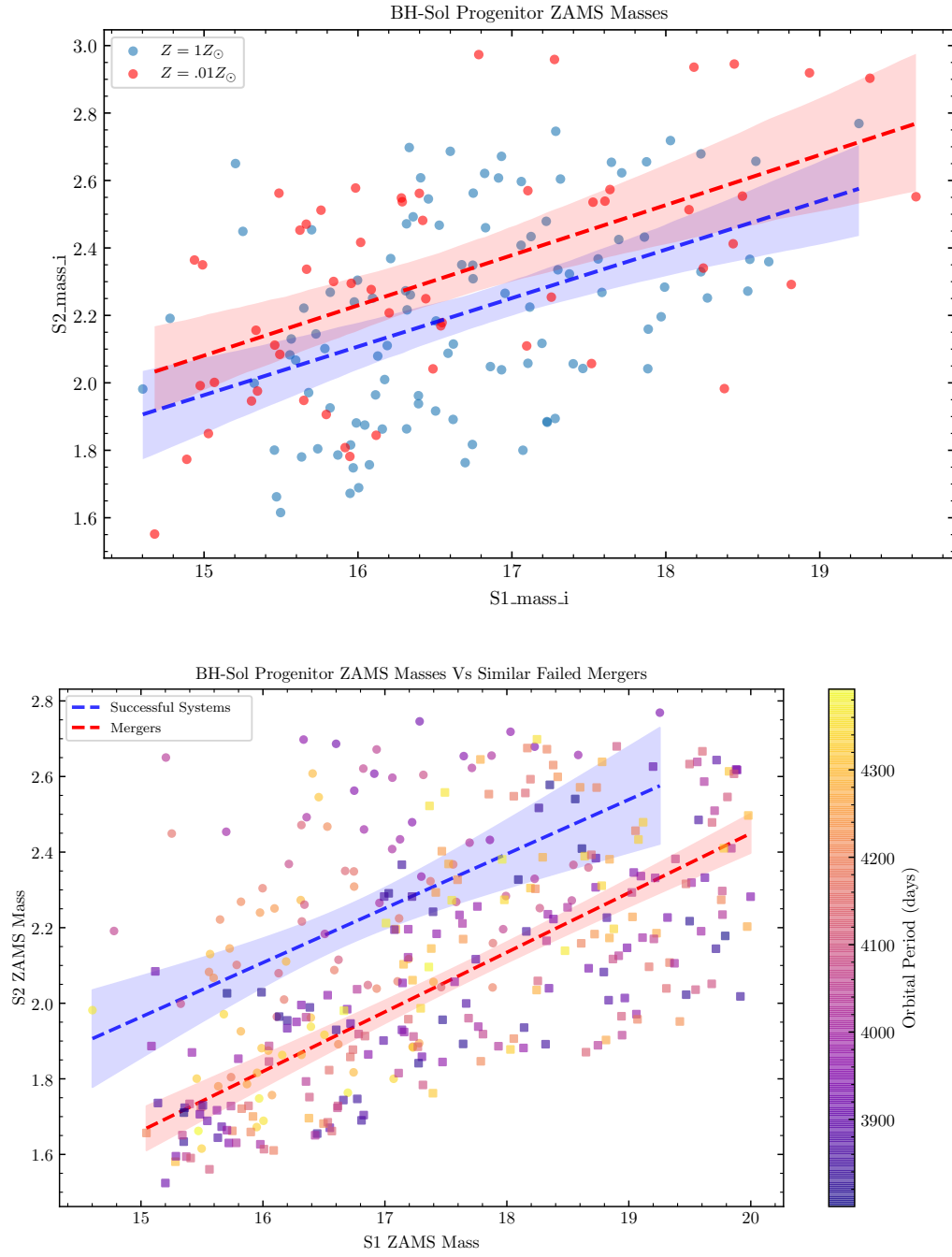
Figure 1: Here we can see that there seems to be a (quite rough) survival line based on the initial mass ratio and the orbital period. Note that these were simply constrained based on the max and min of the initial masses. Next step is actually sampling from a proper matching distribution.
