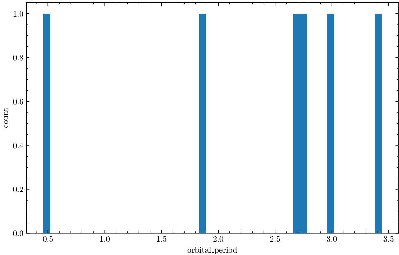
orbital_period of BH-Sol systems at S1 SN
