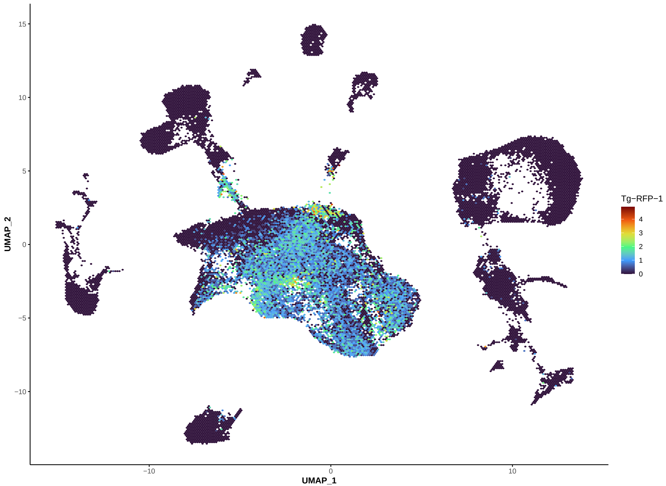
Hexbin Feature Plot: Tg-RFP-1
