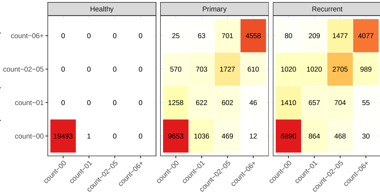
Agreement of RFP probes by sample type
