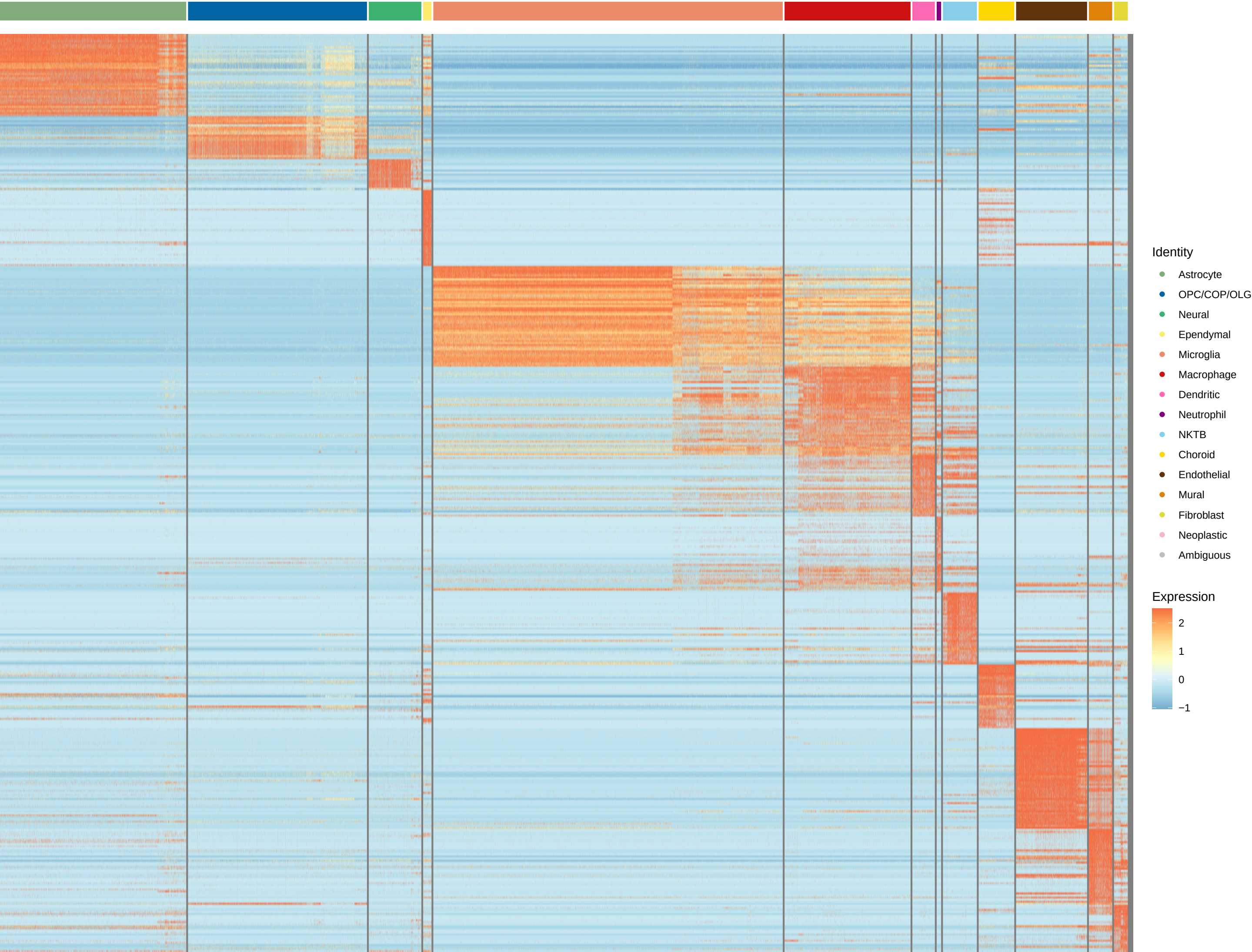
Figure-2E-Heatmap_FindMarkers_NonNeoplastic_Level_3_top50
