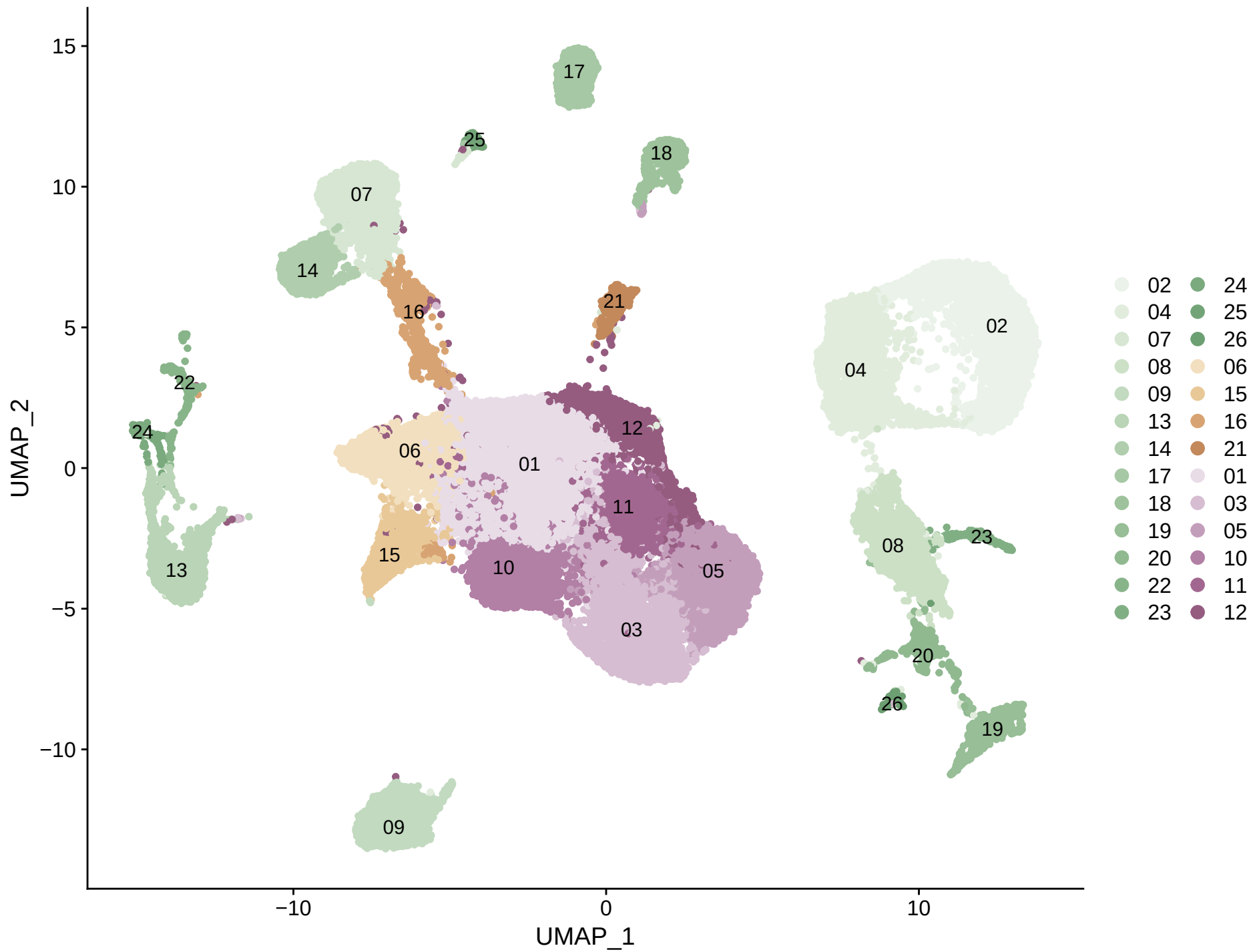
SNN_clusters_all
