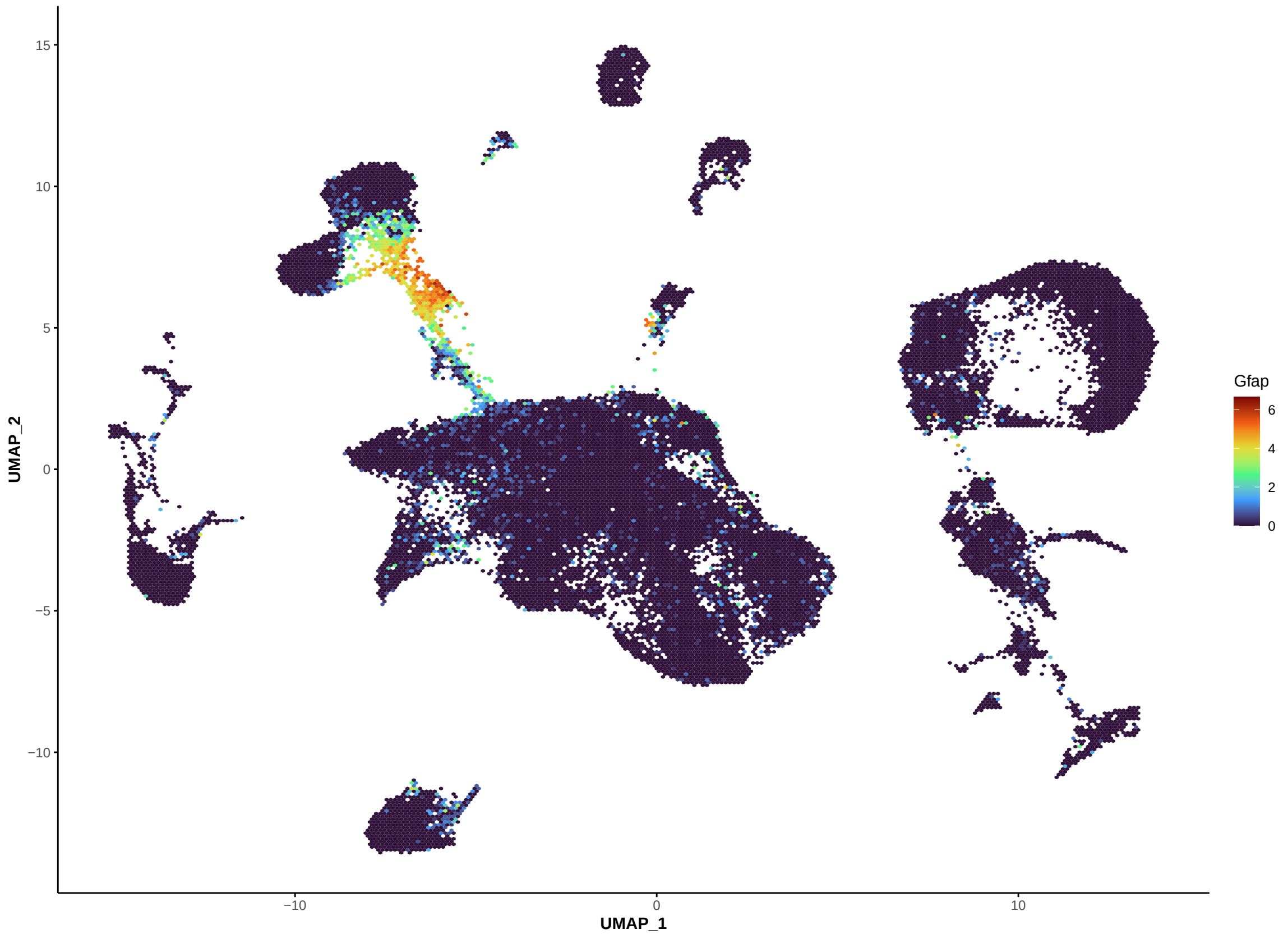
Figure-3-umap-gfap
