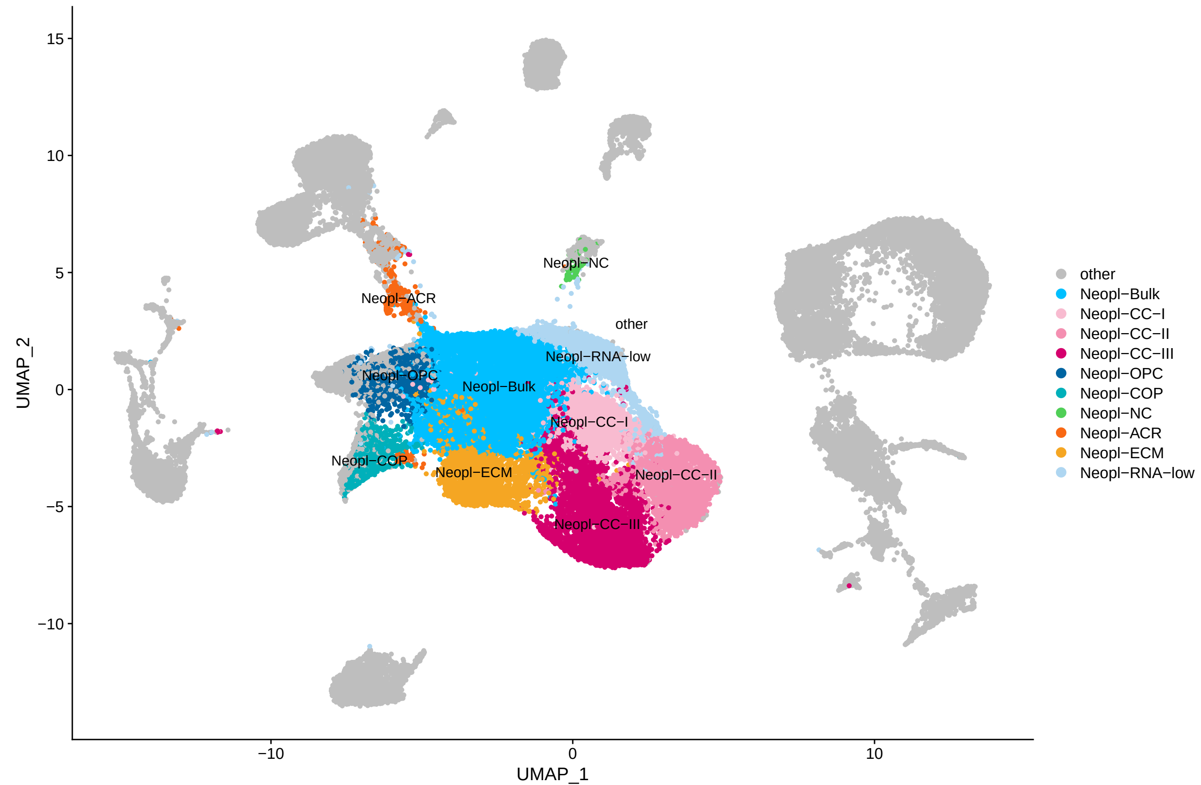
Figure-4-umap-snn-subclusters-neoplastic
