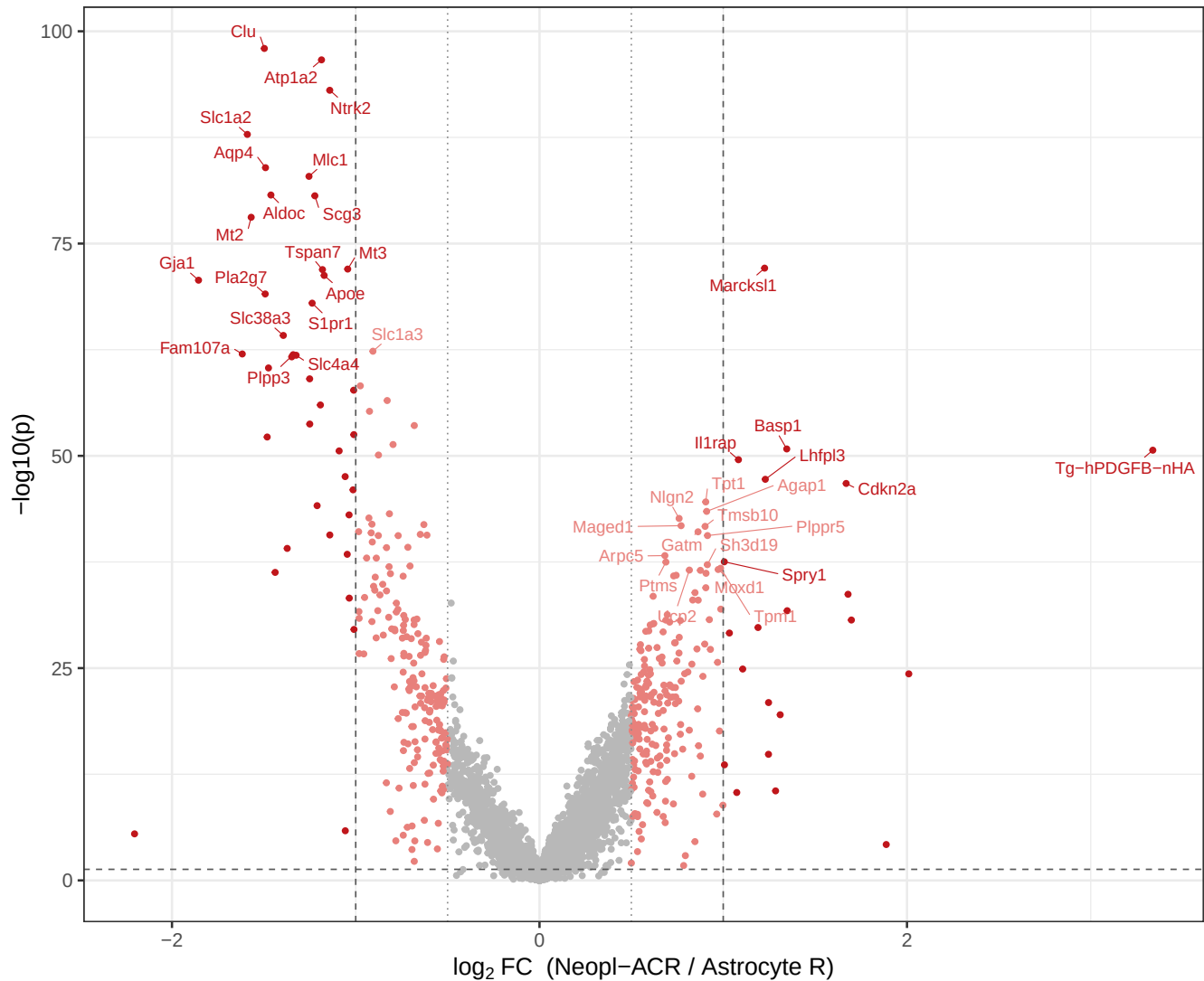
Neopl-ACR vs Astrocyte R
