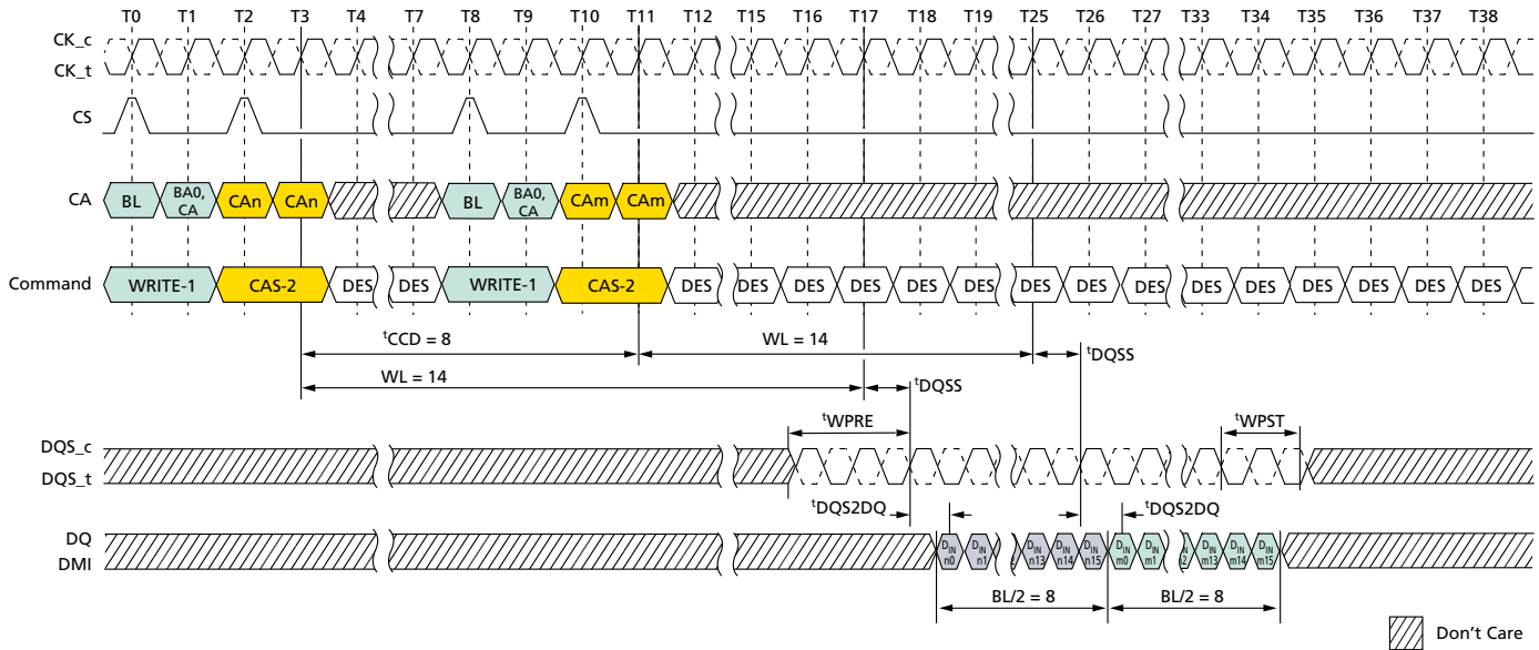
Figure 57: Seamless WRITE: t_{CCD} = \text{MIN} , 1.5nCK Postamble
