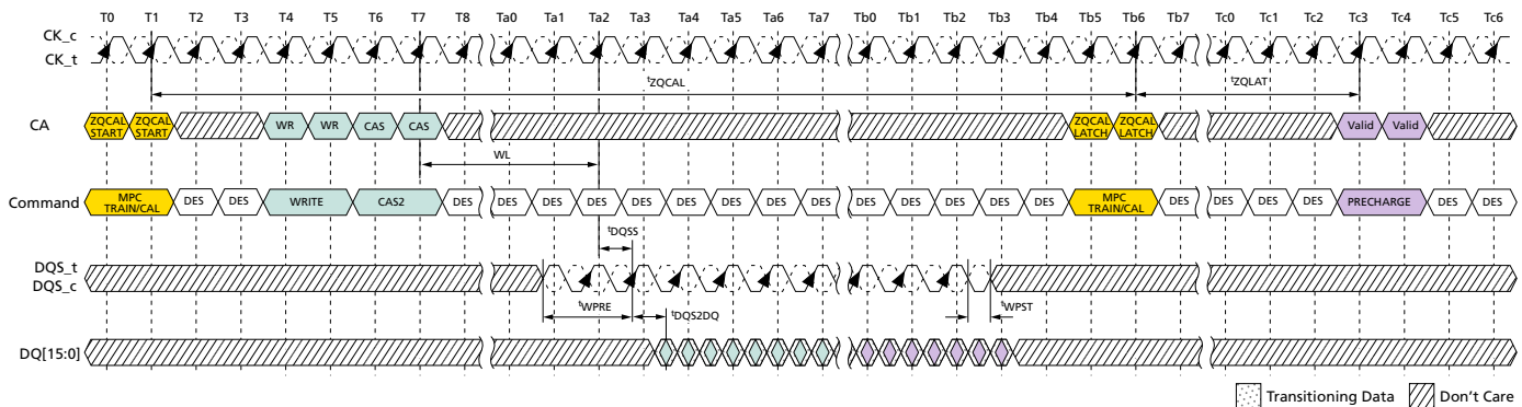
Figure 138: ZQCAL Timing
