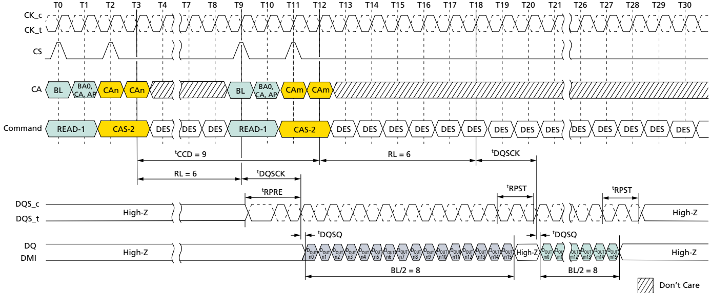
Figure 43: Seamless READ: t_{CCD} = \text{MIN} + 1 , Preamble = Toggle, 1.5nCK Postamble
