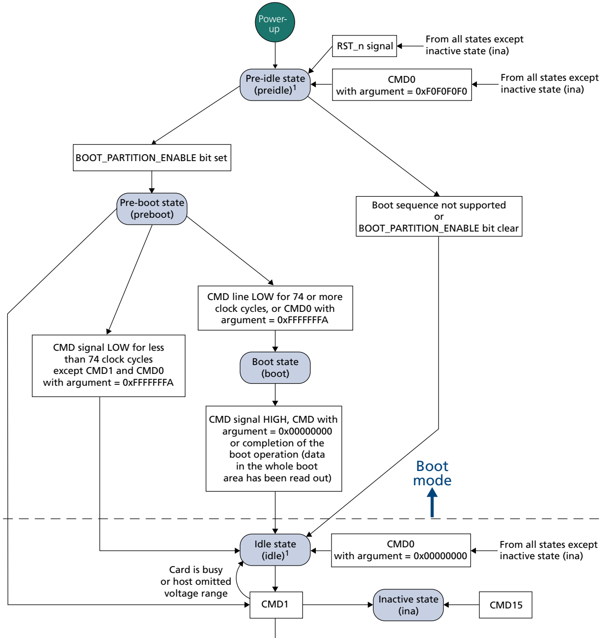
Figure 7: Boot Mode
