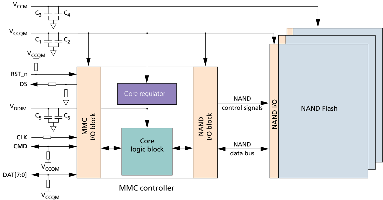
Figure 11: Device Power Diagram
