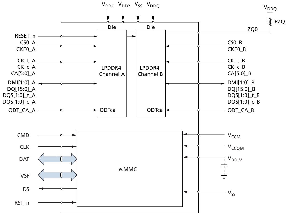
Figure 3: Functional Block Diagram – NAND and Dual-Channel, Single-Rank, Dual-Die LPDDR4X
