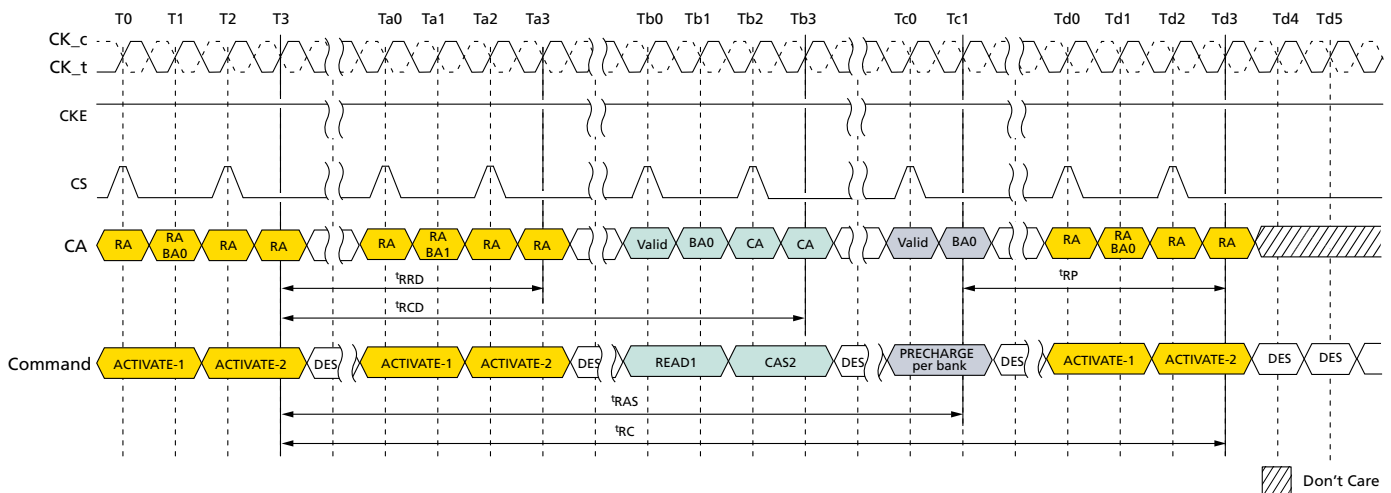
Figure 15: ACTIVATE Command
