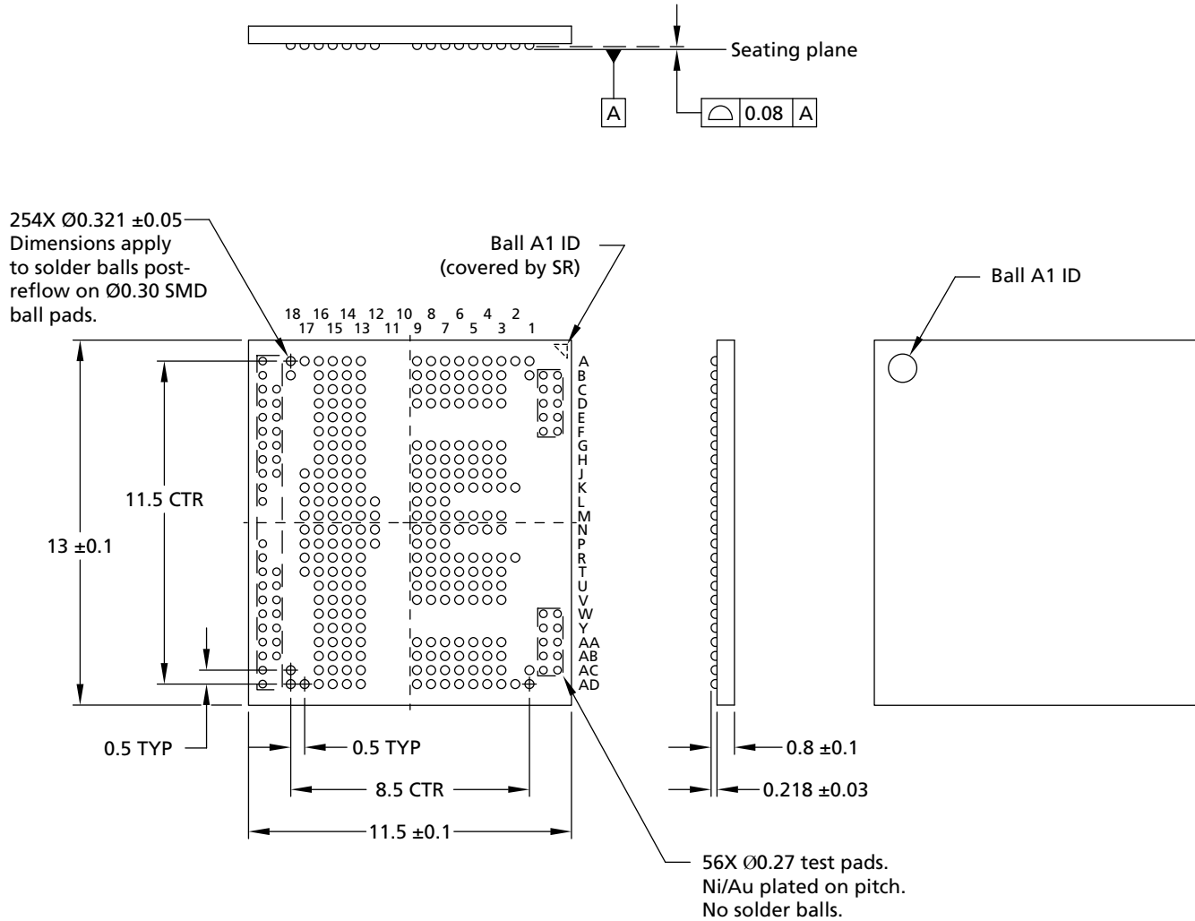
Figure 5: 254-Ball VFBGA (Package Code: SL)
