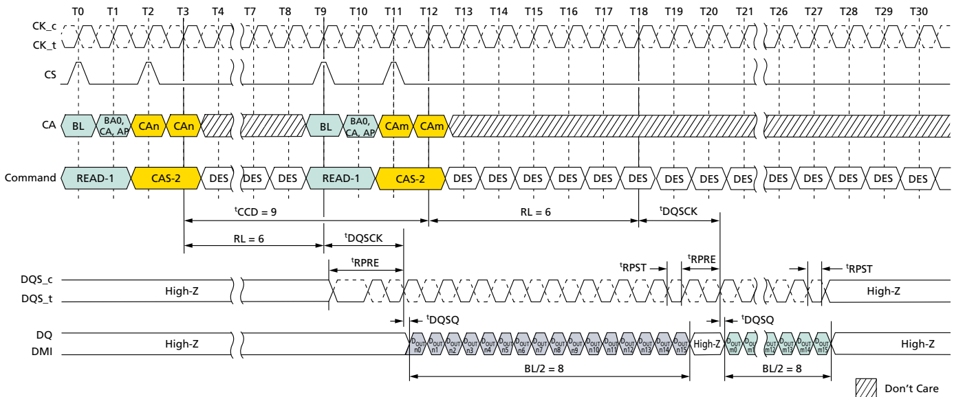
Figure 44: Consecutive READ: t_{CCD} = \text{MIN} + 1 , Preamble = Toggle, 0.5nCK Postamble
