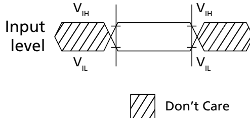
Figure 151: Input Timing Definition for RESET_n
