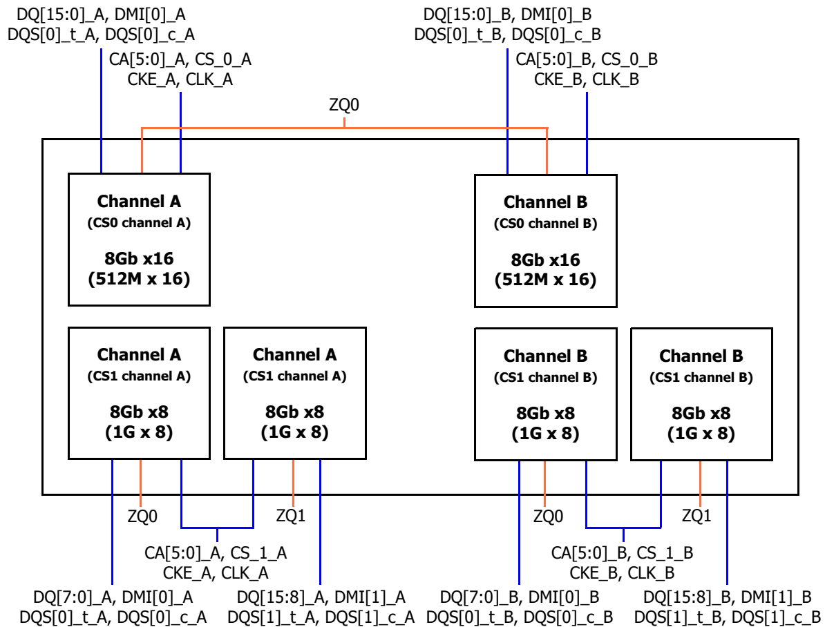
DRAM Block Diagram
