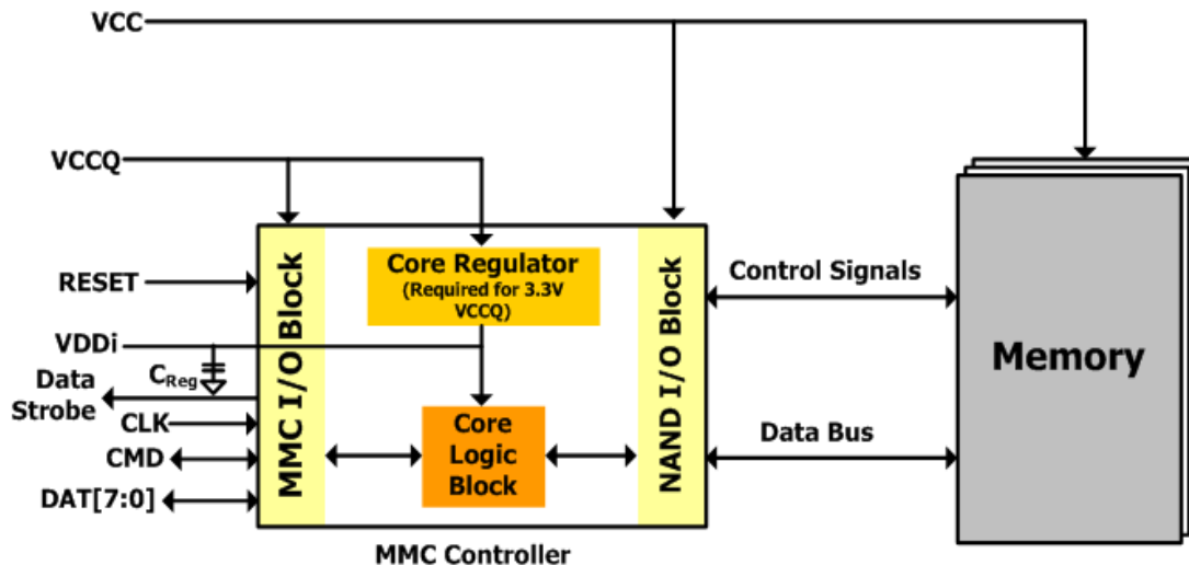
[Figure 15] eMMC internal power diagram
