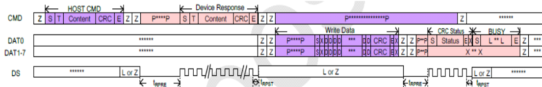
[Figure 9] Enhanced Strobe signals for CMD Response and CRC Response (Write operation)
