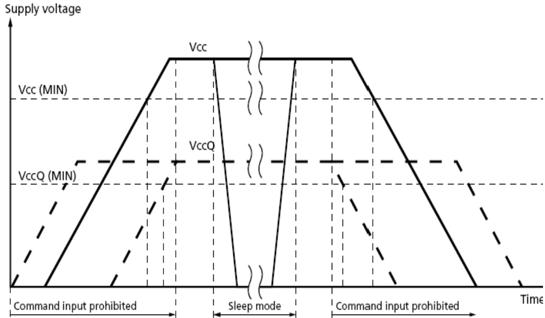
[Figure 19] eMMC power cycle
