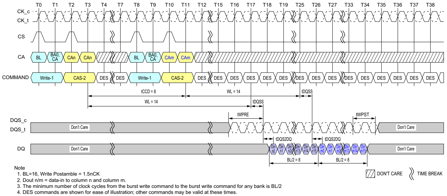
Figure - Seamless Writes Operation: t_{CCD} = \text{Min} , 1.5nCK Postamble
