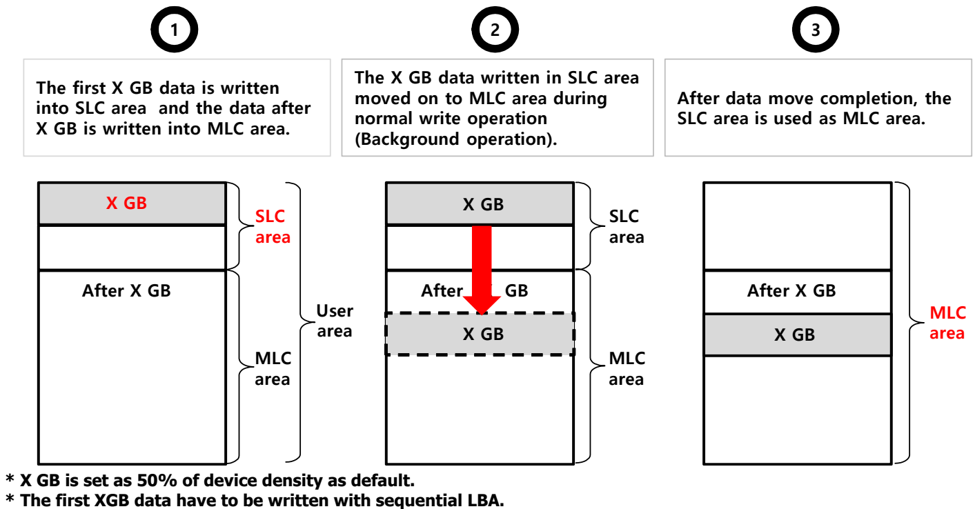
[Figure 8] Pre-coded data protection operation
