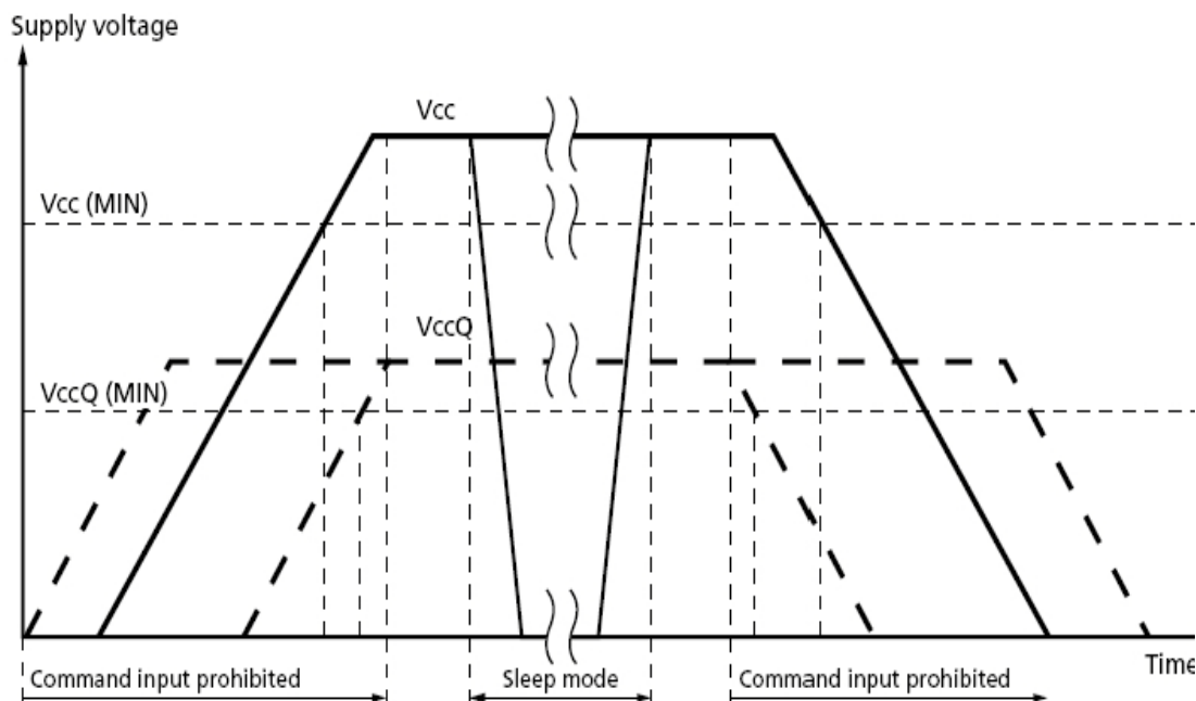
[Figure 13] eMMC power cycle
