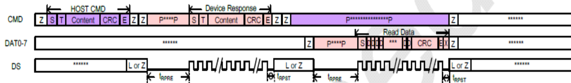
[Figure 7] Enhanced Strobe signals for CMD Response and Data Out (Read operation)
