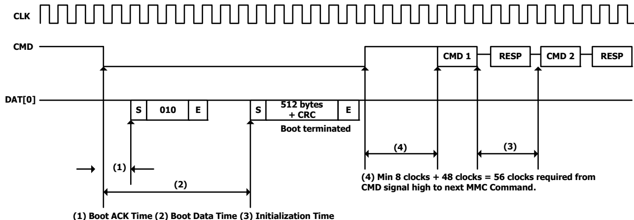
[Figure 16] eMMC state diagram (Boot mode)
