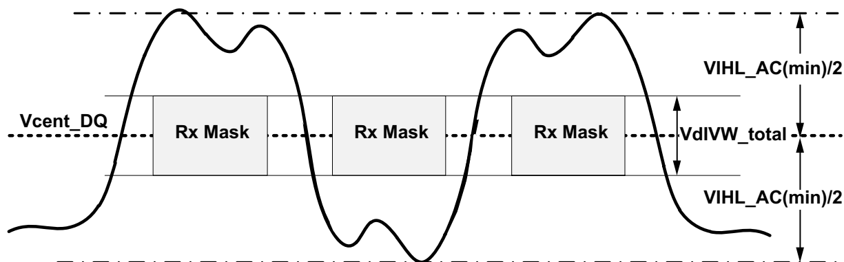
Figure - DQ VIH AC definition (for each input pulse)
