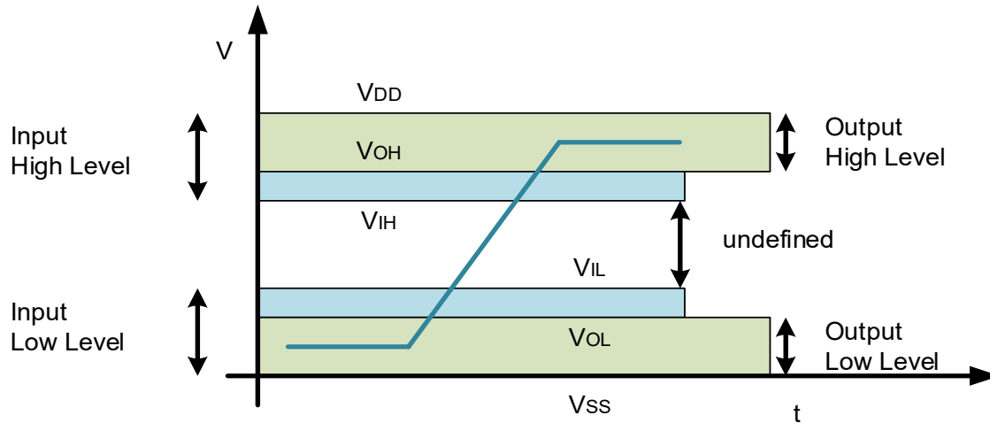
[Figure 14] eMMC bus signal level
