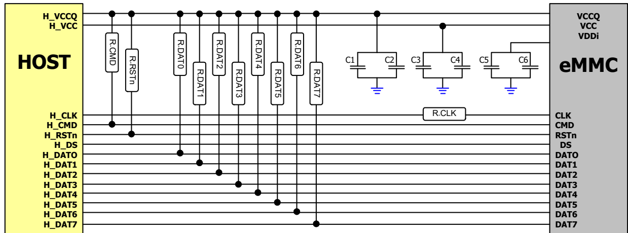
[Figure 14] Connection guide drawing
