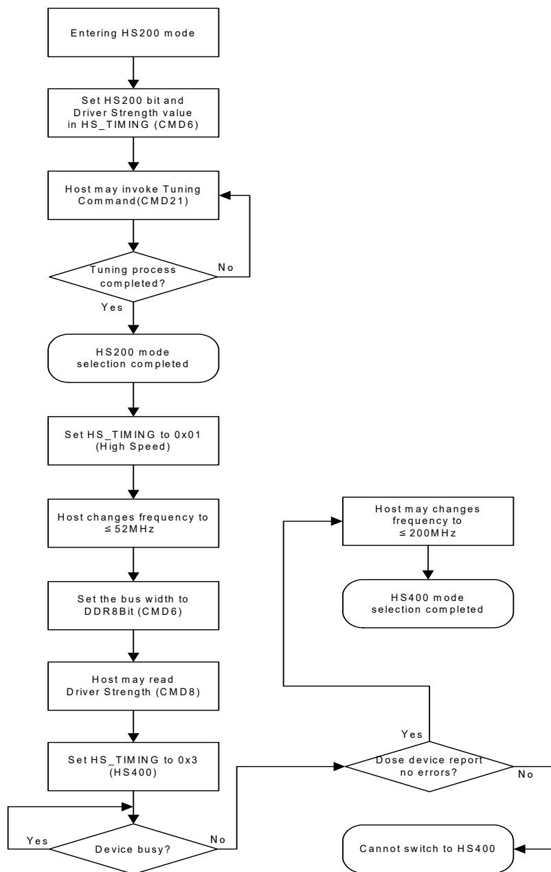
[Figure 4] HS400 Bus mode selection sequence
