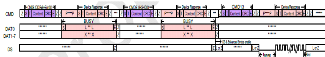
[Figure 9] HS400 mode change with Enhanced Strobe
