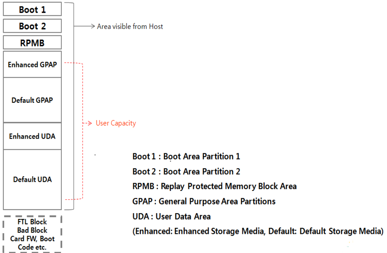
[Figure 15] Partition diagram
