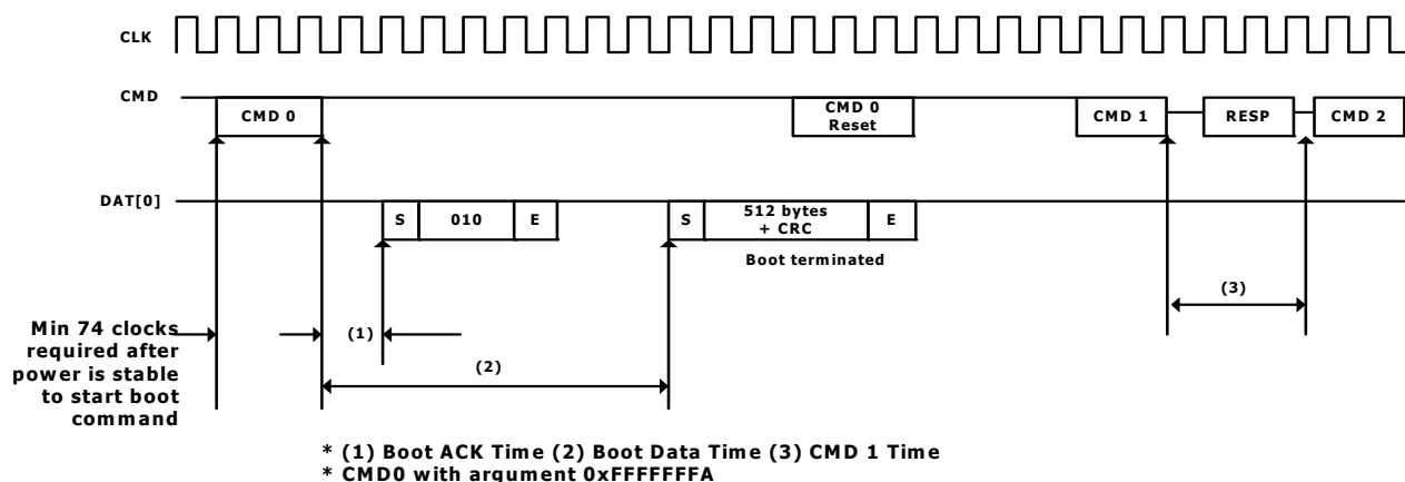
[Figure 17] eMMC state diagram (Alternative boot mode)
