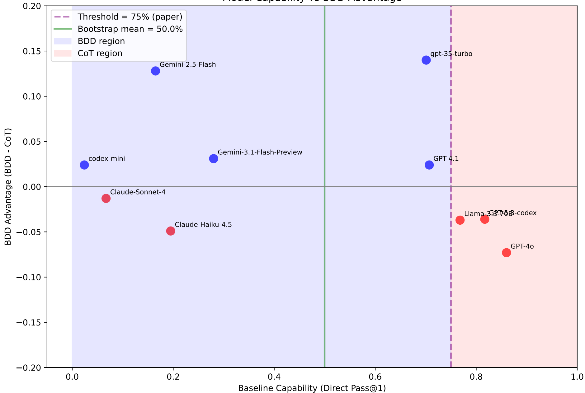
Model Capability vs BDD Advantage
