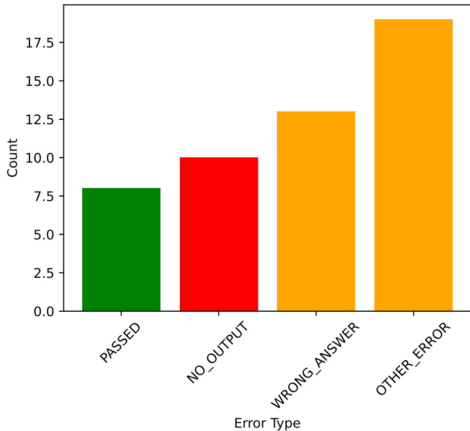
BDD Error Distribution
