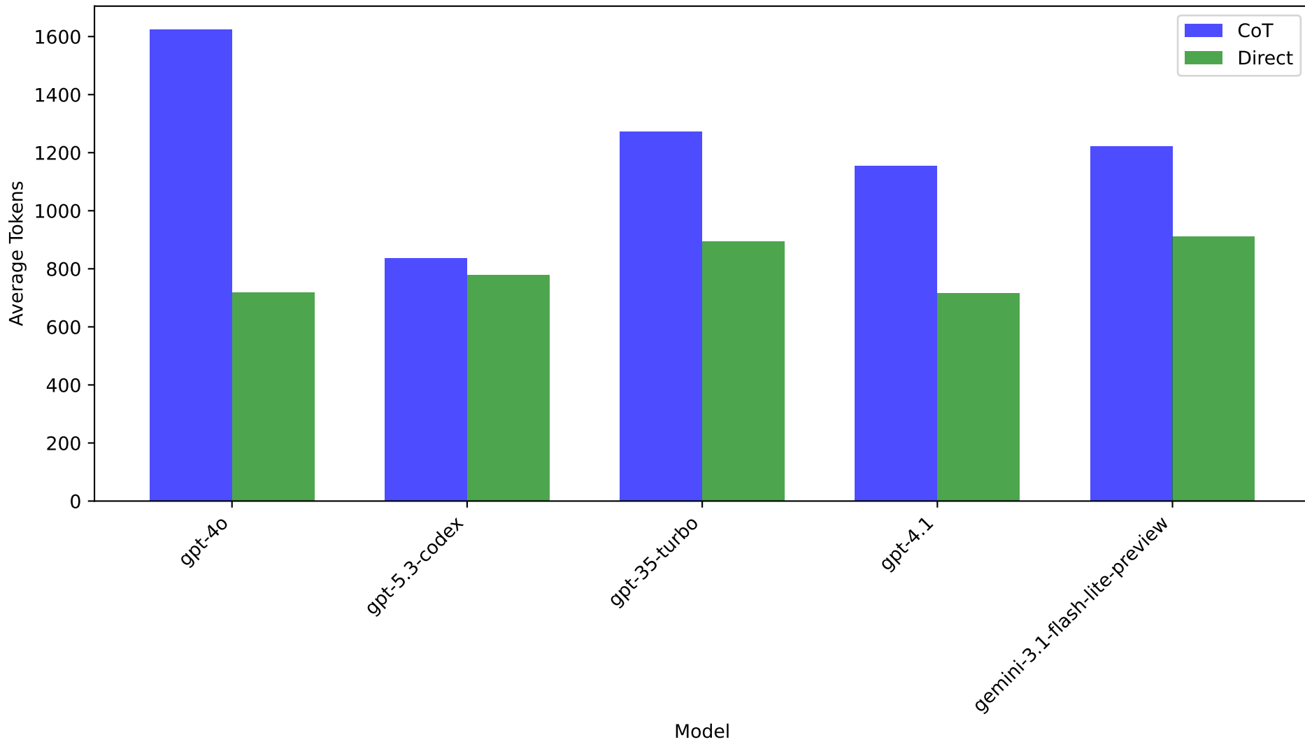
Token Usage: CoT vs Direct on LiveCodeBench
