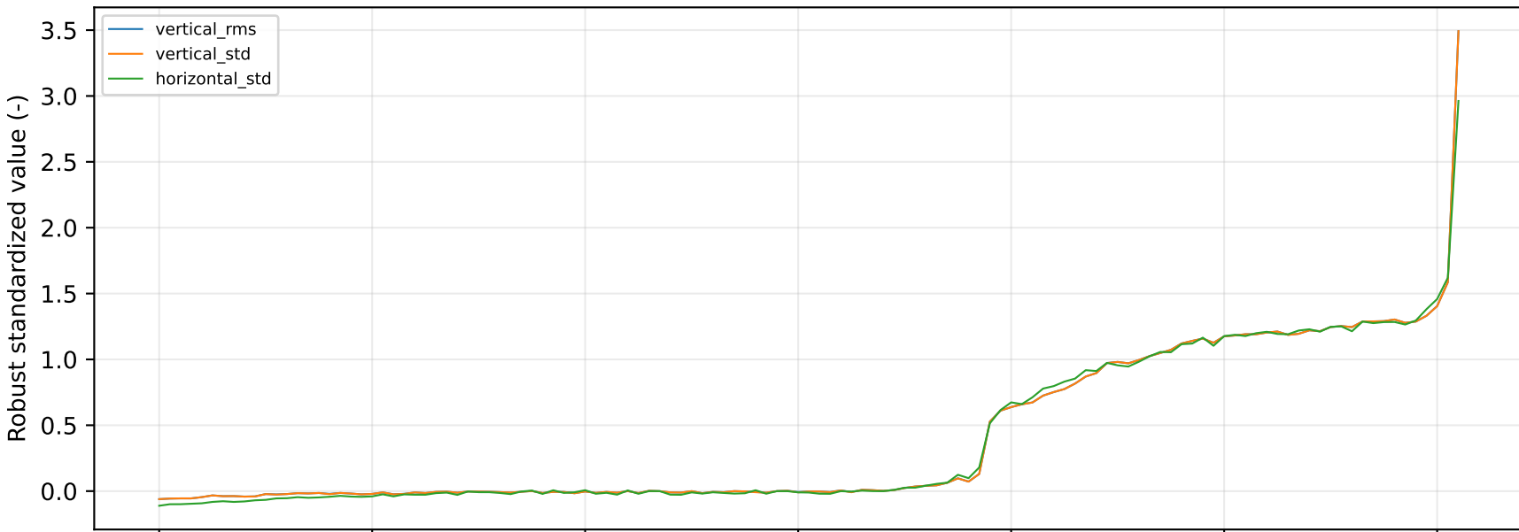
Bearing1_1: degradation-sensitive features
