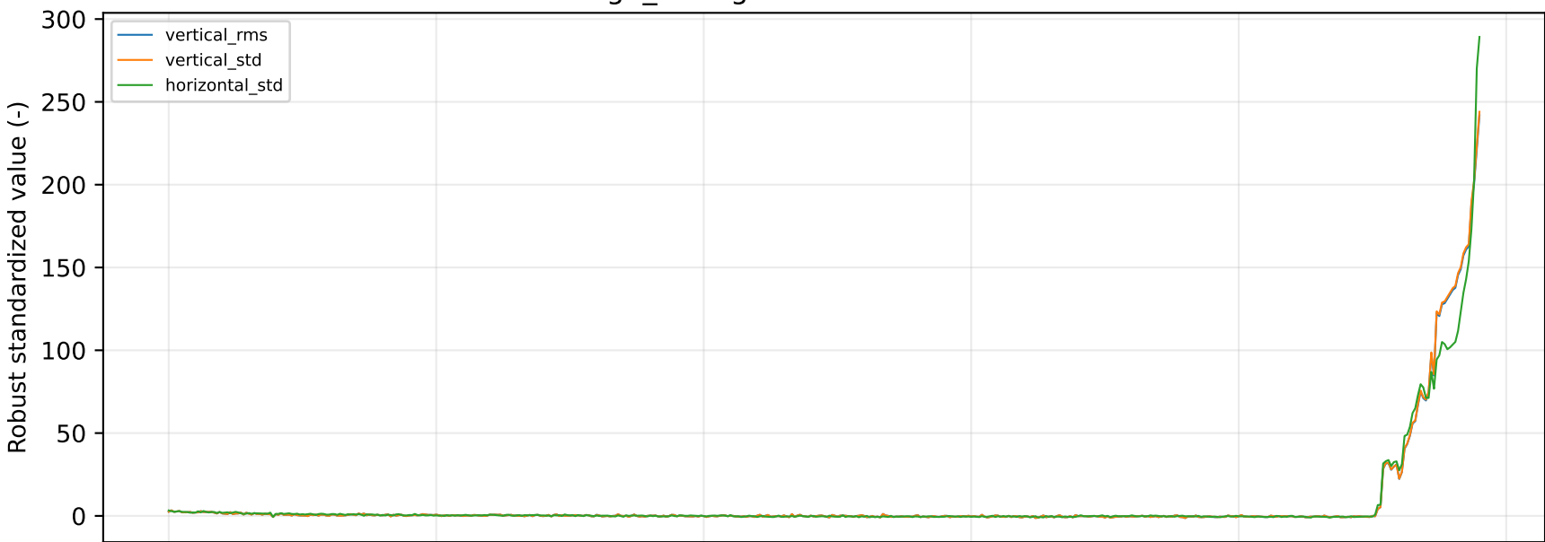
Bearing2_1: degradation-sensitive features
