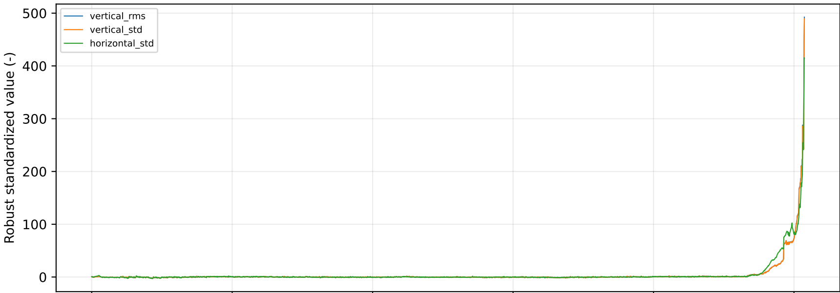
Bearing3_1: degradation-sensitive features
