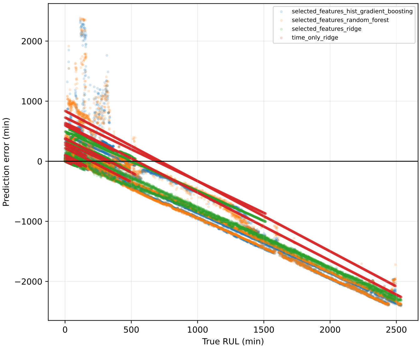
Residuals versus true RUL
