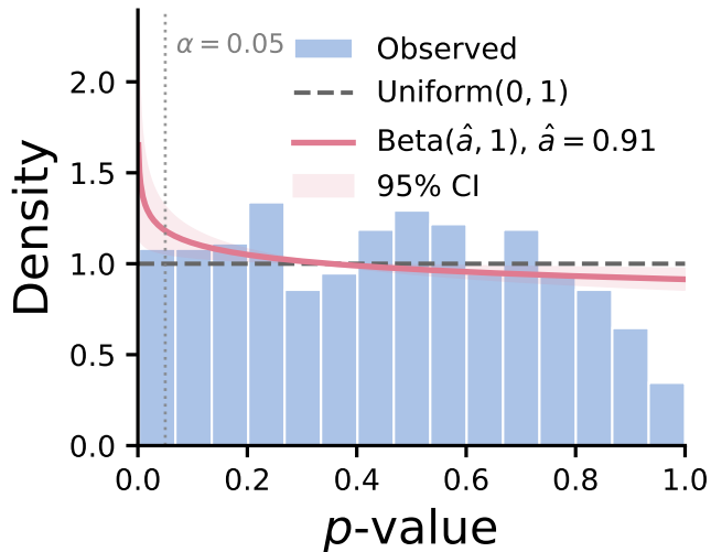
P-value distribution
