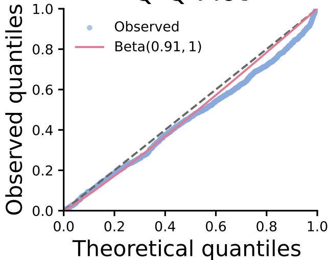
Q-Q Plot
