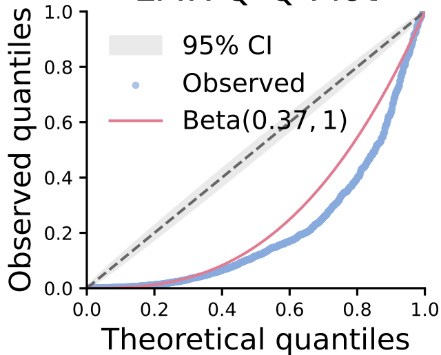
LMR Q-Q Plot
