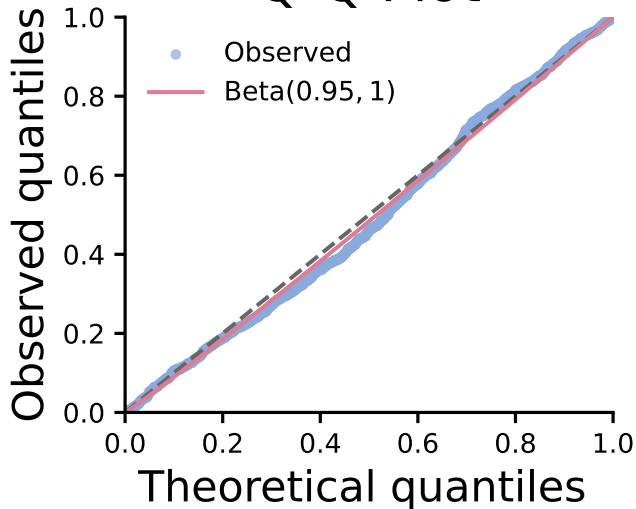
Q-Q Plot
