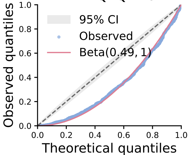
LMR Q-Q Plot
