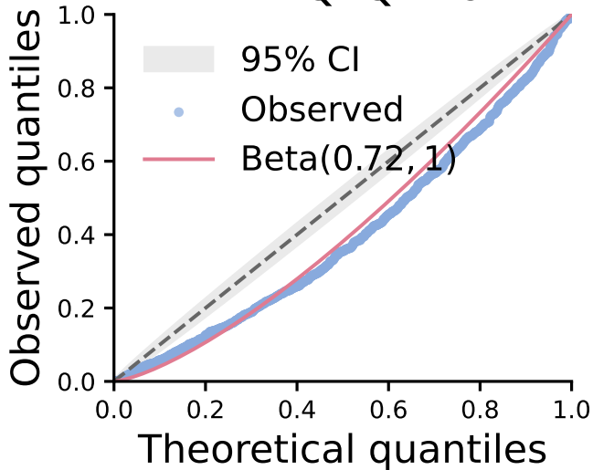
LMR Q-Q Plot
