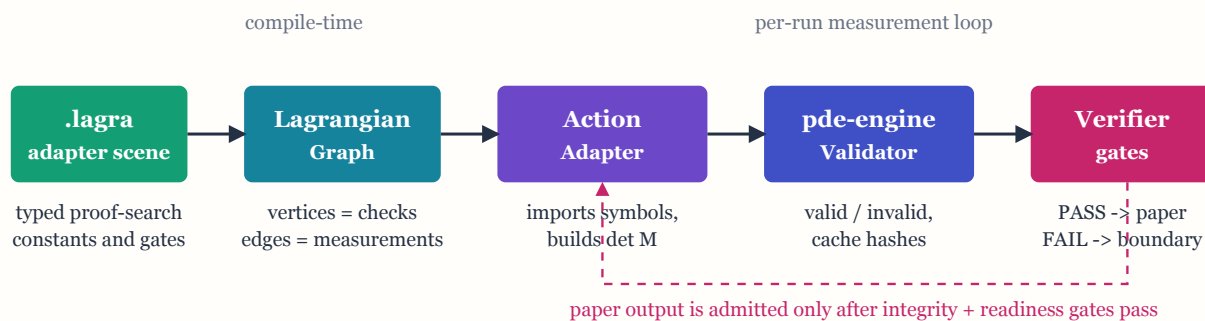
Figure 1: The Lagra/pde-engine adapter pipeline in one figure. This is the direct analogue of the Lagra pipeline figure. The input is a typed Lagra proof-search source plus a local pde-engine checkout. The measured output is not a trajectory; it is a JSON evidence artifact and an admitted paper section. The dashed return path is the strict gate: failed measurements do not become prose.
