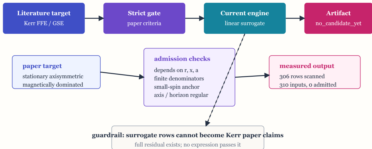
Figure 9: Kerr paper-target gate. The next target uses the same measurement discipline in the negative direction. The bounded Kerr run generated 306 rows; the strict gate scans all rows plus known-anchor and undefined-expression probes against the closed split-monopole nonlinear Kerr Grad-Shafranov residual, then emits no_candidate_yet because no expression passes the criteria.
