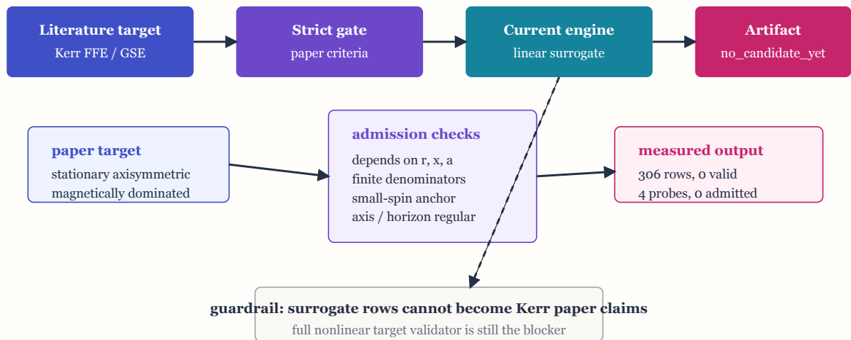
Figure 9: Kerr paper-target gate. The next target uses the same measurement discipline in the negative direction. The bounded Kerr surrogate search generated 306 rows and no valid rows; the strict gate also probes known anchors and a nontrivial anchor-like expression, then emits no_candidate_yet because the repository still lacks the full nonlinear Kerr force-free Grad-Shafranov validator.
