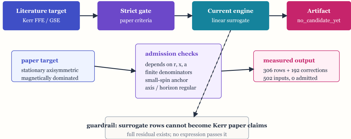
Figure 9: Kerr paper-target gate. The next target uses the same measurement discipline in the negative direction. The bounded Kerr run generated 306 rows; the strict gate scans those rows, 192 targeted finite-spin corrections, and four probes against the closed split-monopole nonlinear Kerr Grad-Shafranov residual, then emits no_candidate_yet because no expression passes the criteria.
