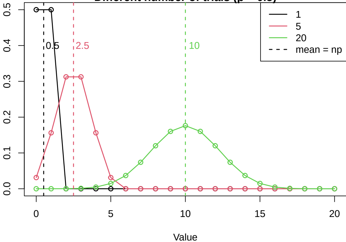
Different number of trials ( p = 0.5 )
