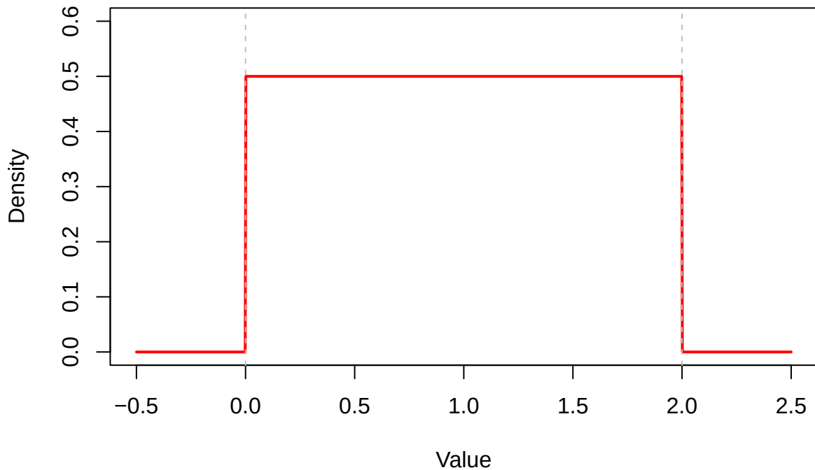
Uniform Distribution ( a = 0 , b = 2 )
