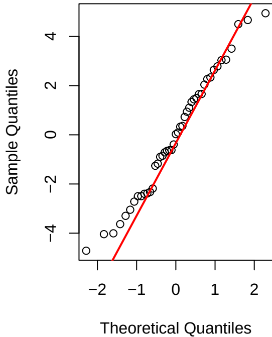
Q-Q Plot of Residuals
