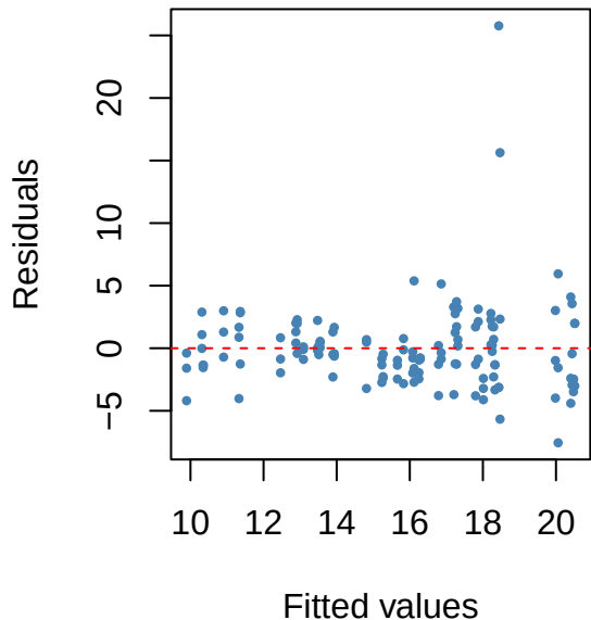
(A) Residuals vs Fitted
