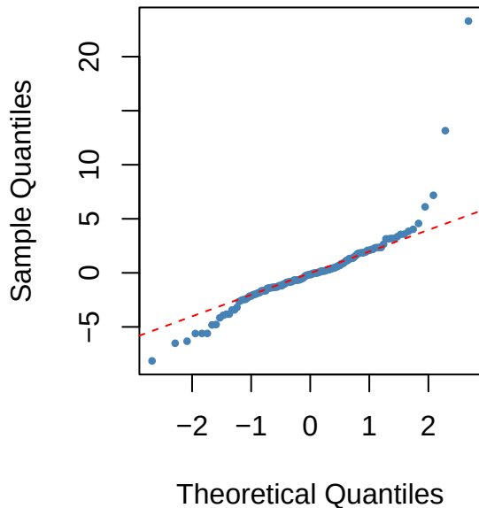
(B) Q-Q Plot of Residuals
