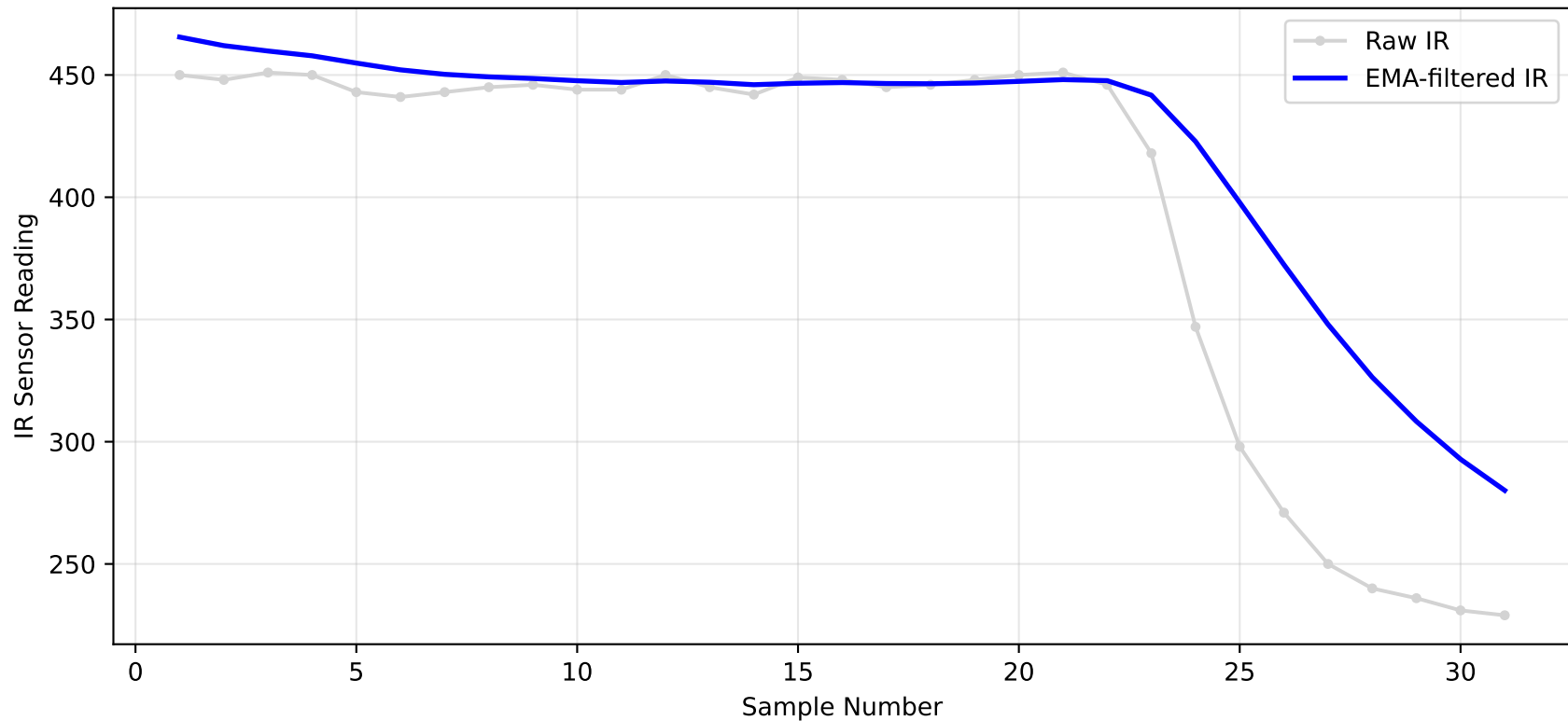
Raw vs. EMA-Filtered IR — Fluorescent
