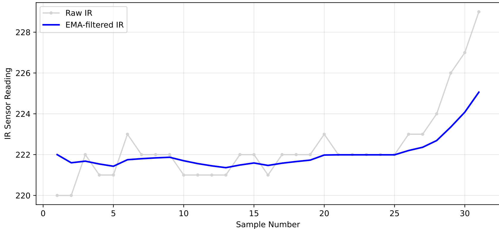
Raw vs. EMA-Filtered IR — Led
