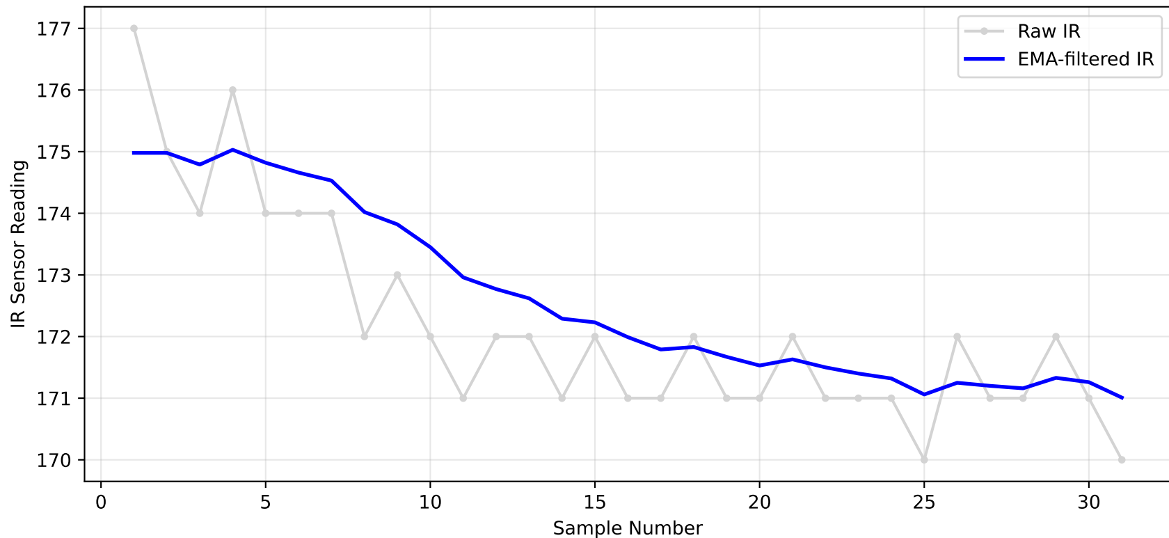
Raw vs. EMA-Filtered IR — Shade
