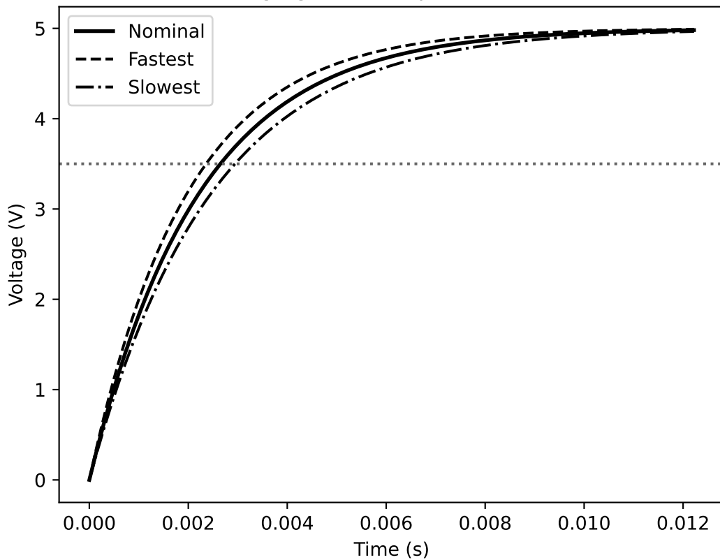
RC charging with component tolerance
